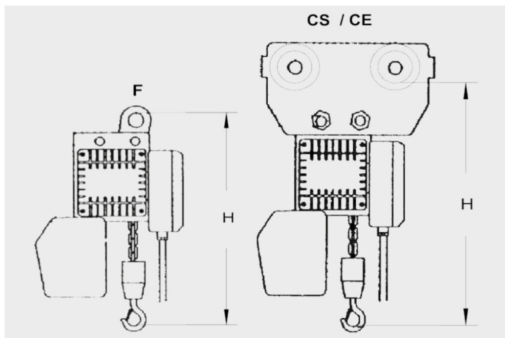
Dimensions mm
