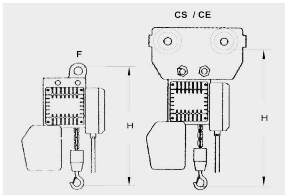
Dimensions mm
