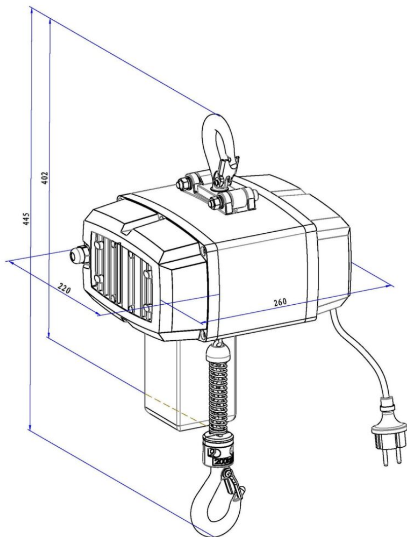
Dimensions TSH-250 / TSH-500
